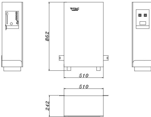
Fig. 5-1 Product Dimensions
