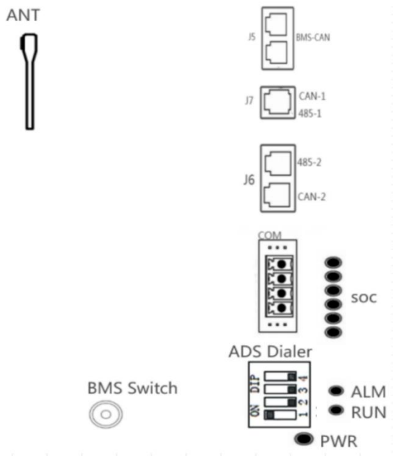
Fig. 5-2 Peration Panel
