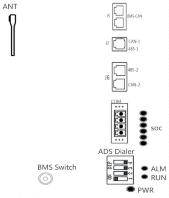
Fig. 5-2 Peration Panel
